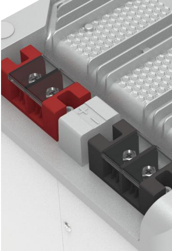
Binding Post
